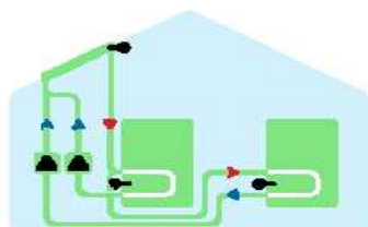
solar + storage tank loading circulating pump
